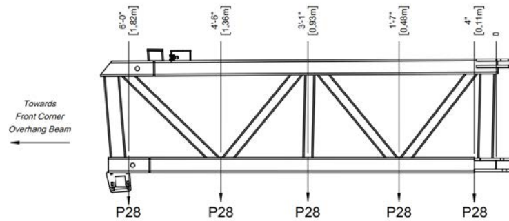
Front corner truss
