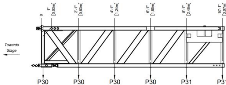
Side overhang truss
