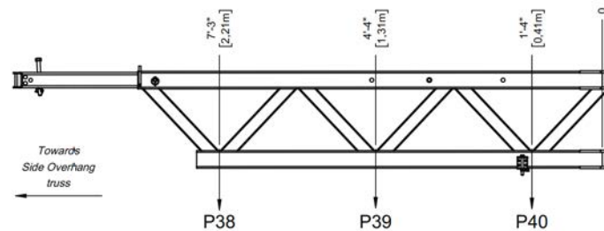
Side truss
